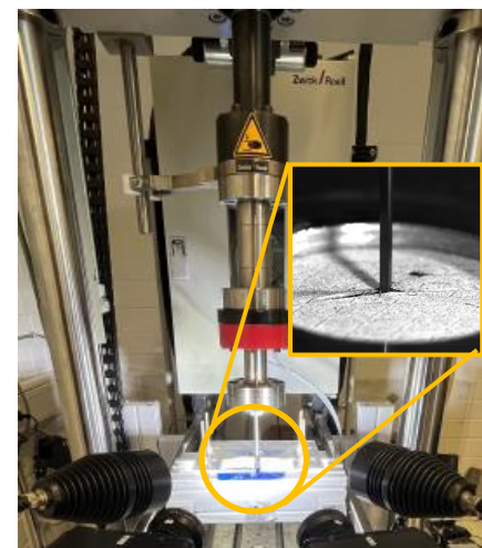
Fig. 2: Stitching Material characterization
