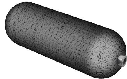
Fig. 1: Hydrogen Pressure Vessel
